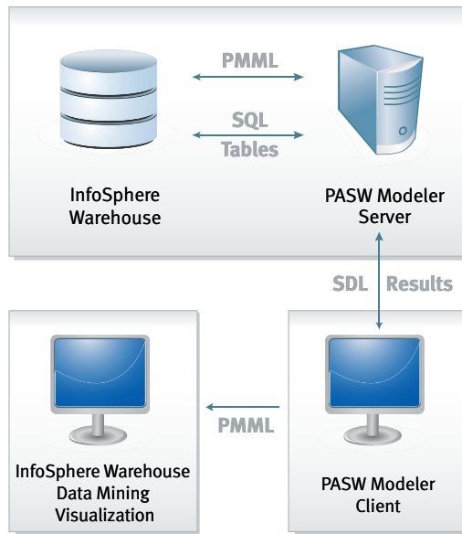
Figure 1: PASW Modeler is completely integrated with your IBM InfoSphere Warehouse solution.
